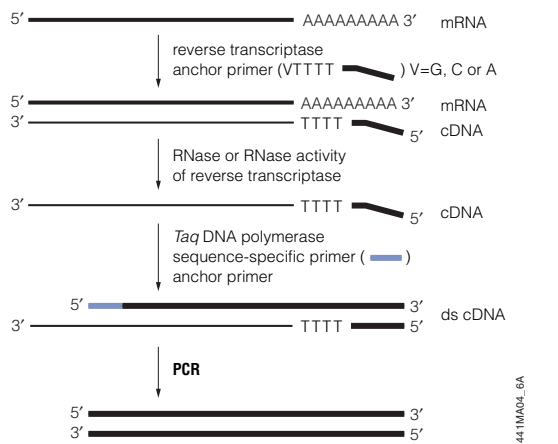
Figure 1.5. Schematic diagram of a typical 3'-RACE protocol.
