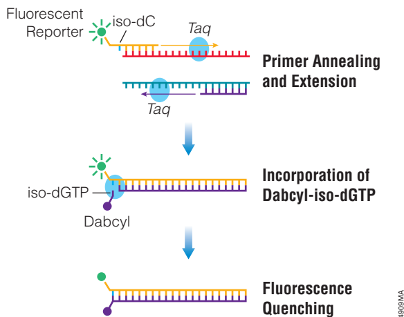
Figure 1.3. Quenching of the fluorescent signal by dabcyI during product accumulation.
